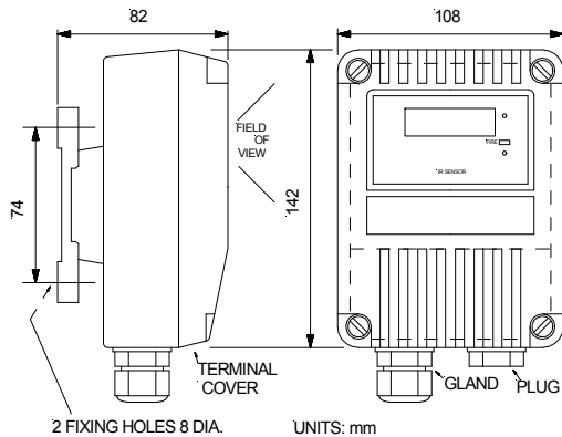
Fig. 8 Dimensions – IR 3 Flame Sensor (Gland not supplied)
