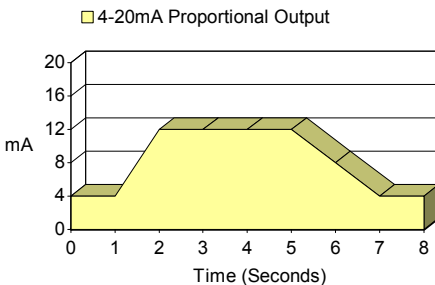
Fig. 7 Typical Response to Burst of Flame - IR 2 Flame Sensor
