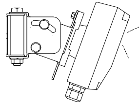
Fig. 9 Adjustable Mounting Part number: 007127
